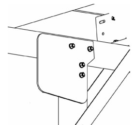
Fastening with optional inverter plate
