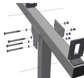
Fastening with connecting plate
