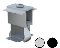
MC AK II Klick 30-50 with grounding plate
